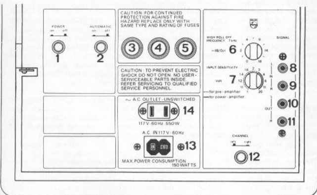
Figure 2, Rear Panel
